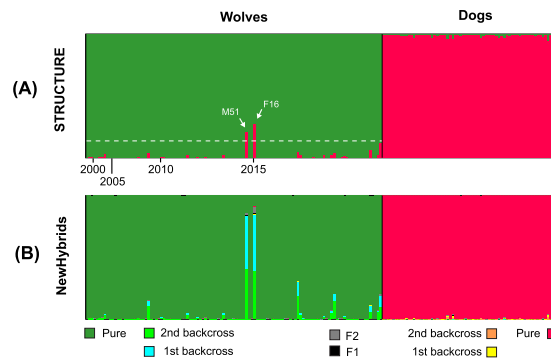
Figure 2. Bayesian clustering of individual wolf and dog genotypes (A) with STRUCTURE into two groups, and (B) with NewHybrids into eight genotype classes, including six hybrid and two parental classes ( n = 99 pure wolves and 55 pure dogs). Individuals are arranged by their time of first detection. The dotted line show the threshold computed from analyses of simulated hybrids (Fig. S1). The two individuals above this threshold are shown.
